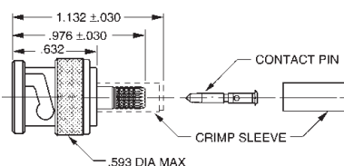
BNC UPL220 Series
